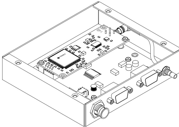
Figure 1-1. The Module Installed Inside the Interface Unit
