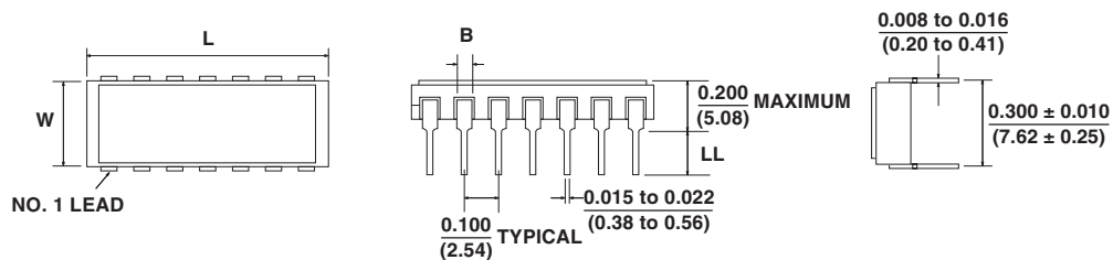
FIGURE 1 - PACKAGE SIZES AND CHARACTERISTICS
