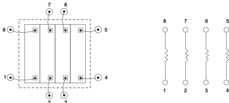
FIGURE 2 - SAMPLE CIRCUIT DESIGN AND CHIP LAYOUT
