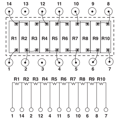
TEN RESISTOR DIVIDER
