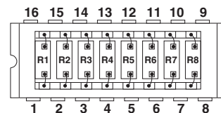
EIGHT RESISTOR PACKAGE
