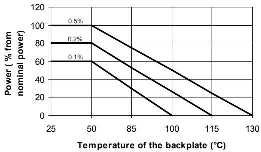
FIGURE 2 – DERATING
