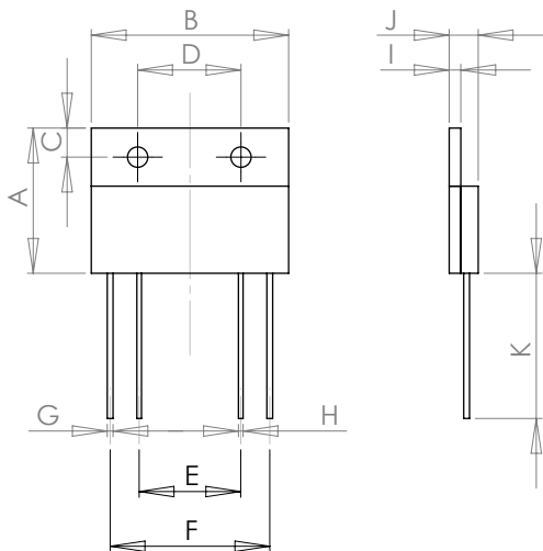
FIGURE 3 – DIMENSIONS in mm (inches)
