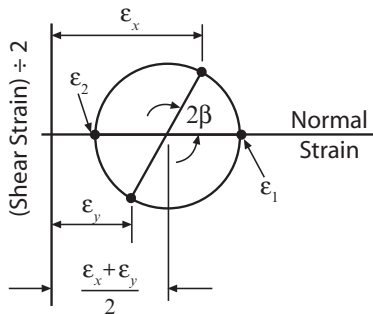
Figure 1. Mohr's circle of strain, illustrating the equivalence of (\epsilon_x + \epsilon_y)/2 and (\epsilon_1 + \epsilon_2)/2 .
