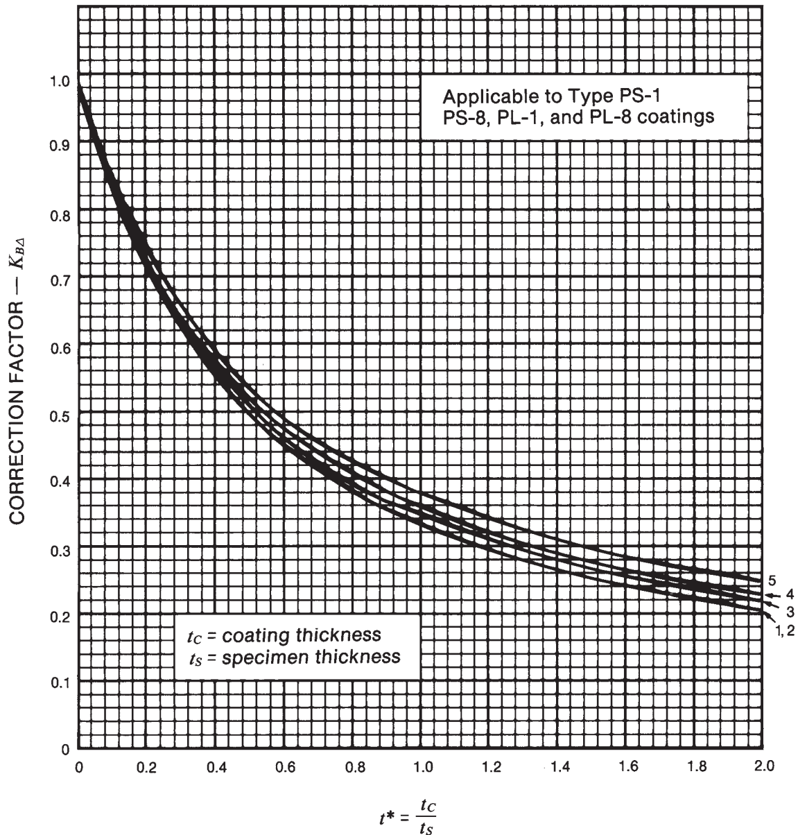
Figure 6. Correction factor K_B (imposed curvature) for Separator Gage. Multiply the Separator Gage strain measurement by the appropriate factor to obtain the correct strain. Refer to KEY in Figure 5 B for Specimen Elastic Modulus, E_s .
