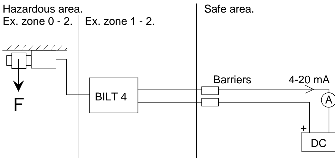
Figure 2. With BILT 4 and the transducer in a hazardous area, the cable to the instrumentation in the safe area must pass through protective barriers.
