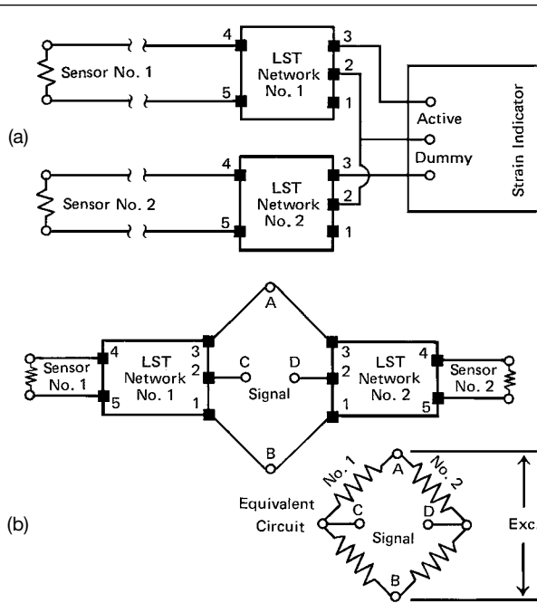
Figure 7. Differential temperature measurement using two TG sensors and two LST networks – (a) half-bridge arrangement and (b) full-bridge arrangement.
