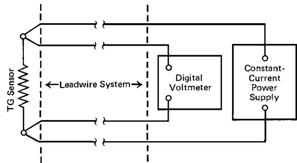
Figure 3. Four-wire circuit for TG sensor.
