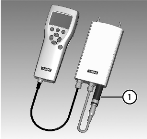
Figure 1. Correct connection of GM70PUMP
