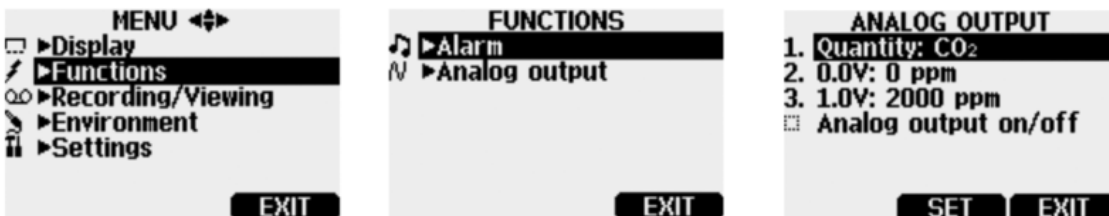
Figure 1. Selecting analog output
