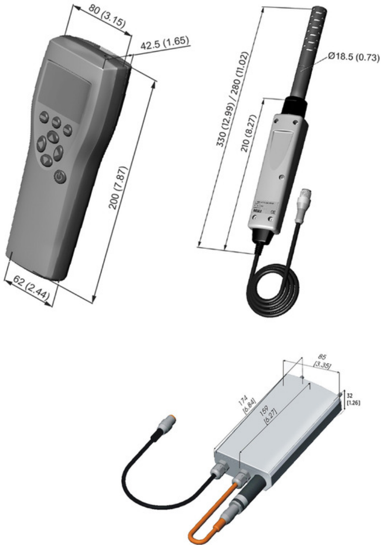
Figure 1. GM70 dimensions in mm (in)
