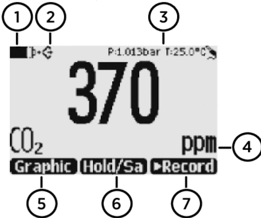
Figure 1. GM70 basic display
