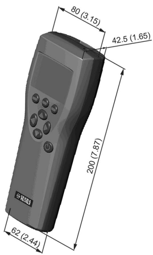
Figure 21 MI70 Indicator
