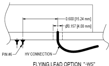
FLYING LEAD OPTION "-WS"
