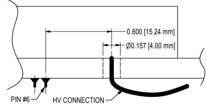
FLYING LEAD OPTION
