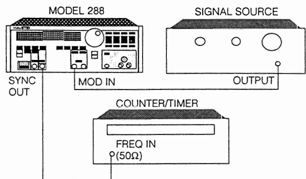
Figure 2-3. VC/FM Setup
