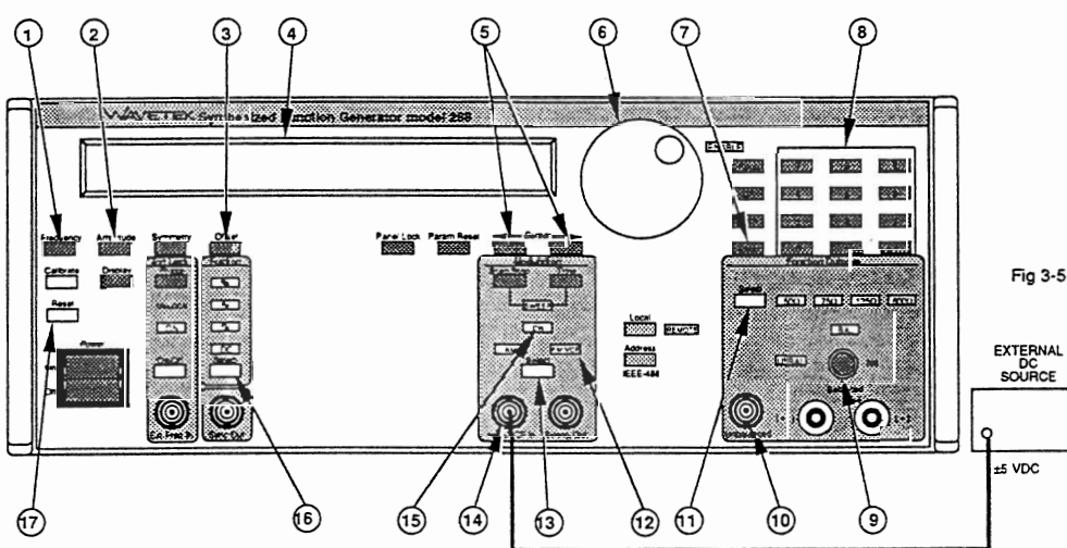
Figure 3-7. VCF Operation Control Setup
