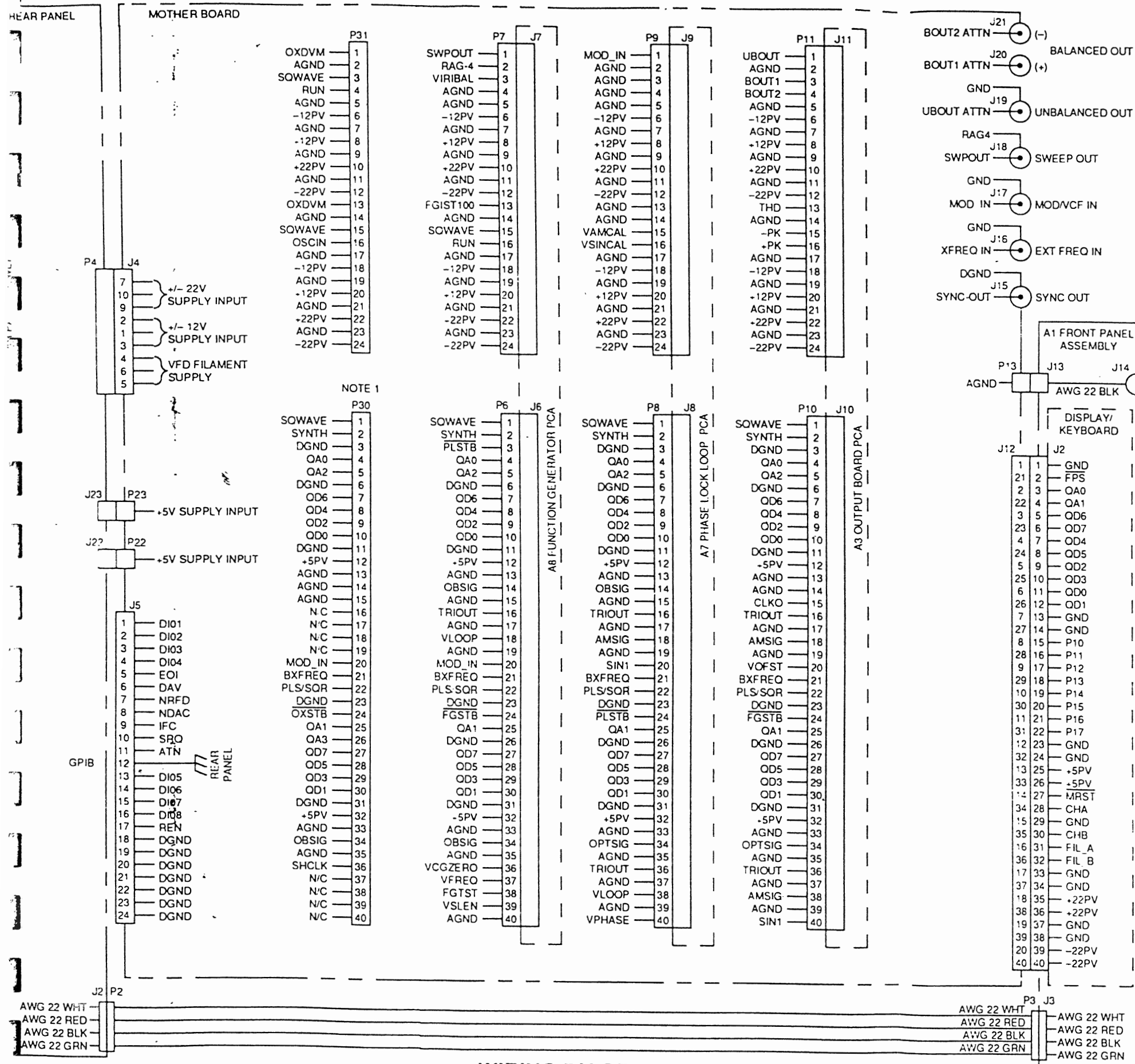
WIRING DIAGRAM
