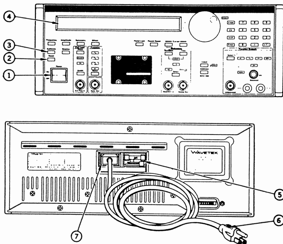
Figure 2-1. Equipment Setup
