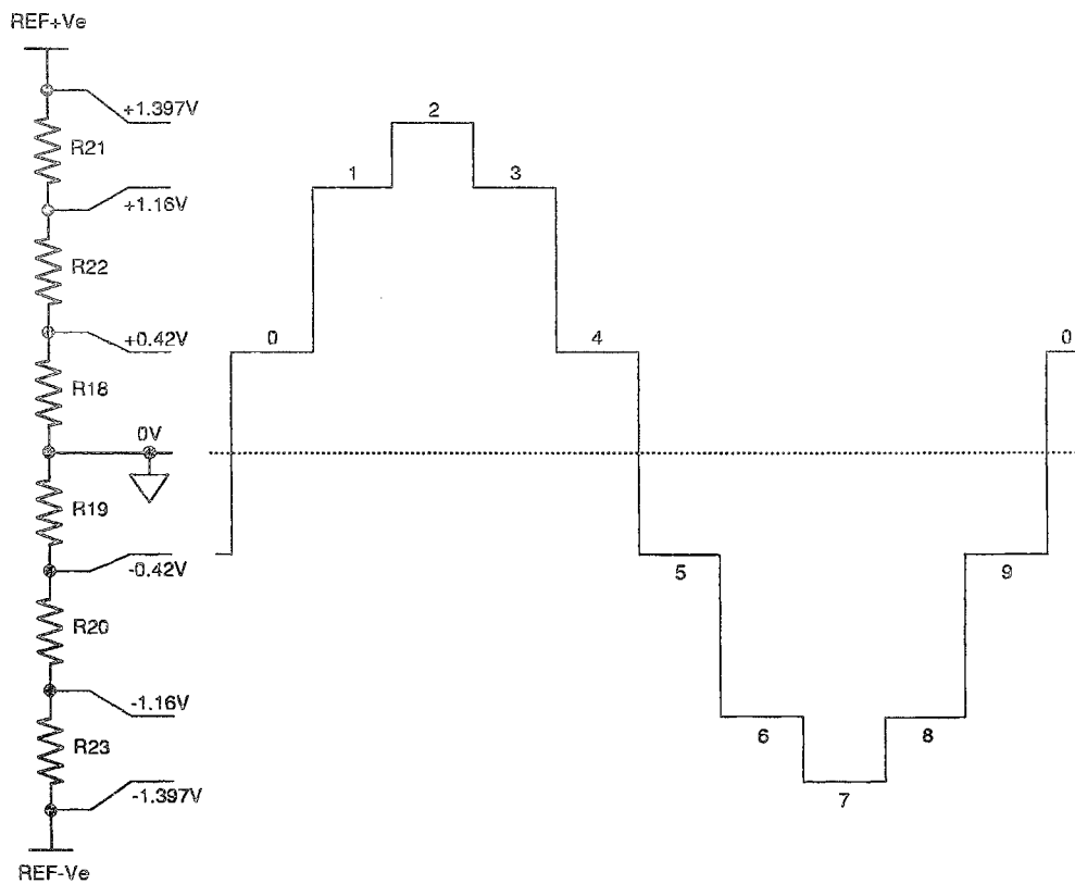
FIG. 6.28 QUASI-SINEWAVE GENERATION
