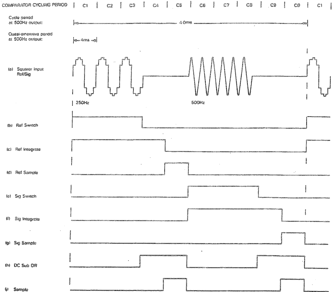
FIG. 9.12 SINE/QUASI-SINE COMPARATOR - SEQUENCE TIMING
