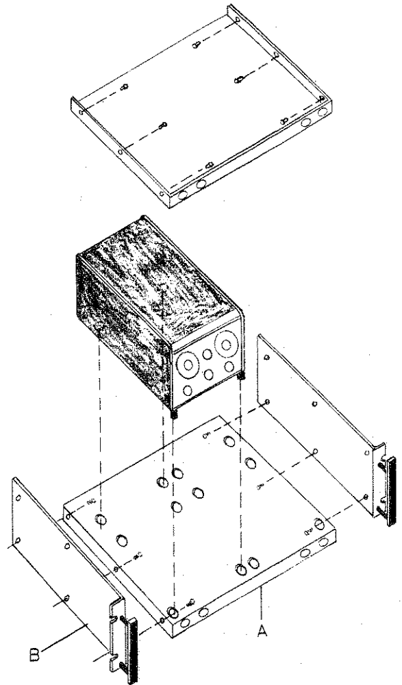
Figure 2-2. K-104 Rack Mounting
