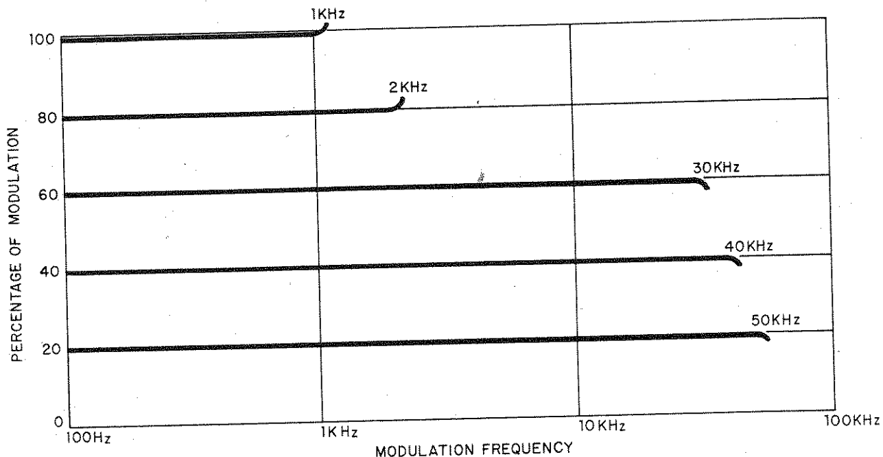
Figure 3-7. Percentage Modulation/Modulating Frequency
