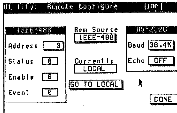
Figure 4-82. Remote Screen
