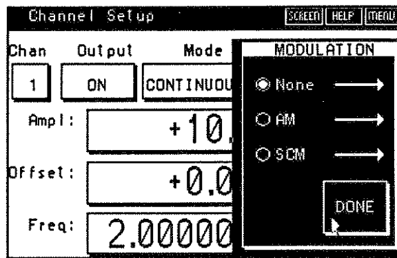
Figure 4-14. Modulation Menu
