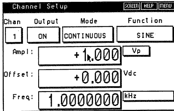
Figure 2-14. Changing Amplitude
