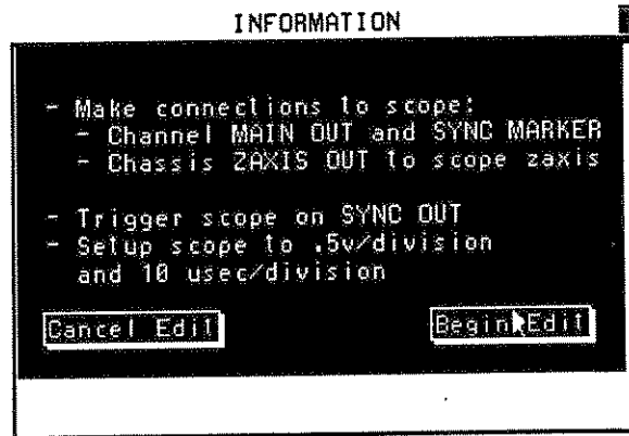
Figure 4-32. Information Screen
