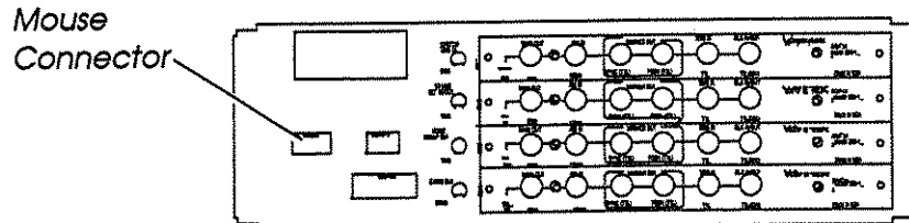
Figure 2-3. Mouse Connection
