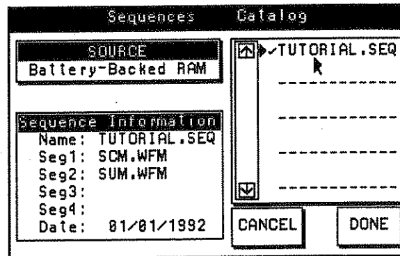
Figure 4-49. Sequence Catalog
