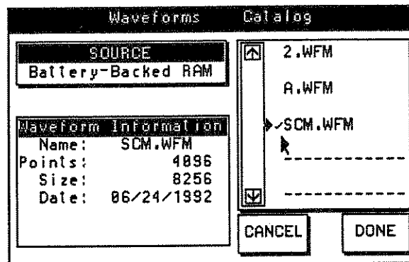
Figure 4-7. Waveforms Catalog
