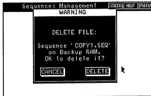
Figure 4-62. Warning Screen
