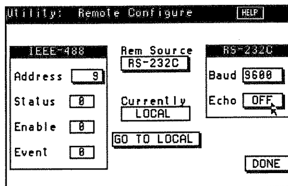
Figure 5-4. RS-232 Screen
