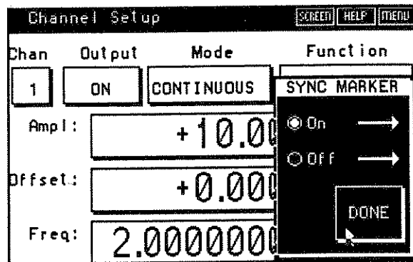
Figure 4-19. Sync Marker
