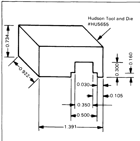
FIGURE 24 — Shield Preparation
