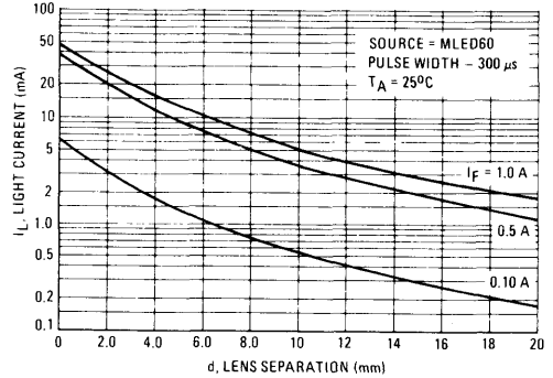
FIGURE 5 – PULSED LIGHT CURRENT versus DISTANCE
