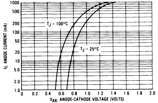
FIGURE 2 — ANODE CURRENT versus ANODE-CATHODE VOLTAGE
