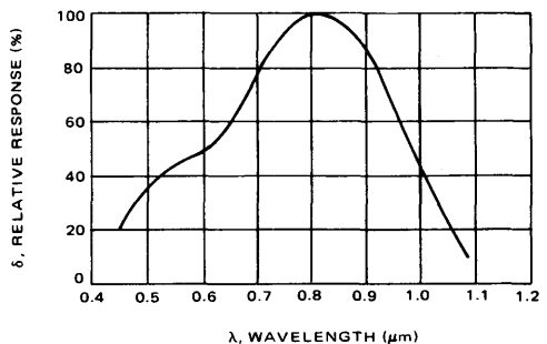
FIGURE 9 - Constant Energy Spectral Response for MRD300
