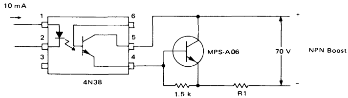
FIGURE 10 – TYPICAL TELETYPE INTERFACE
