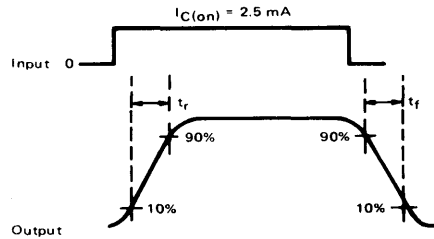
FIGURE 5 – VOLTAGE WAVEFORM
