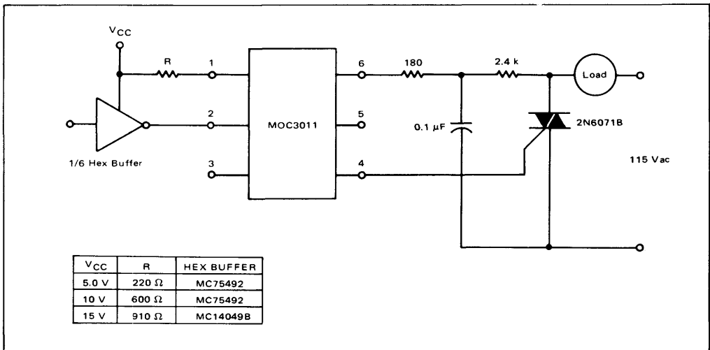
FIGURE 6 – MOS to ac Load Interface
