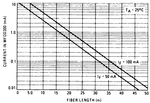
FIGURE 4 – MFOE200 SOURCE
