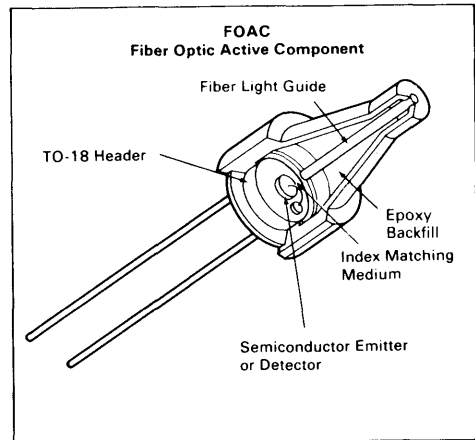
FIGURE 2 — FOAC Construction
