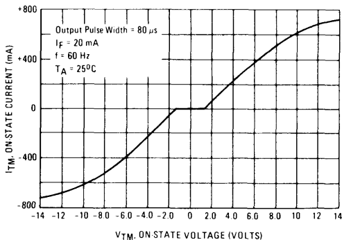
FIGURE 1 – ON STATE CHARACTERISTICS
