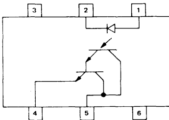
FIGURE 1 – DEVICE SCHEMATIC
