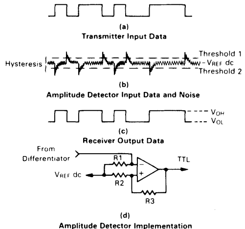
FIGURE 14 — Edge Detector Operation
