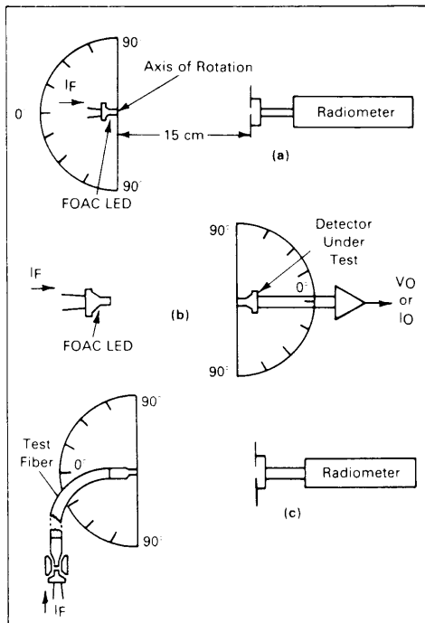
FIGURE 11 — NA Measurement
