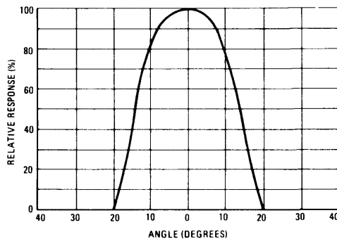
FIGURE 9 – ANGULAR RESPONSE
