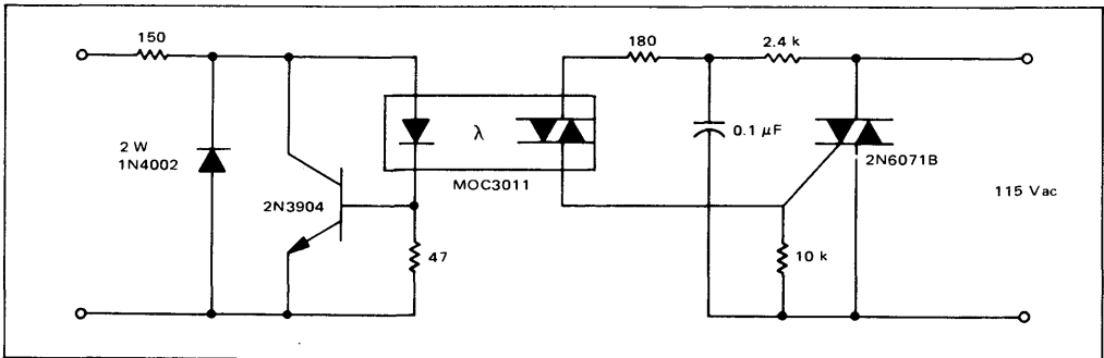
FIGURE 10 — Solid-State Relay
