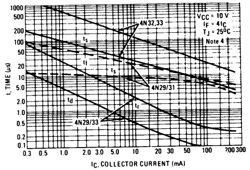
FIGURE 7 - SWITCHING TIMES
