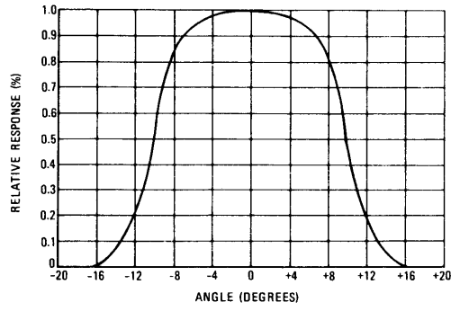
FIGURE 8 – ANGULAR RESPONSE
