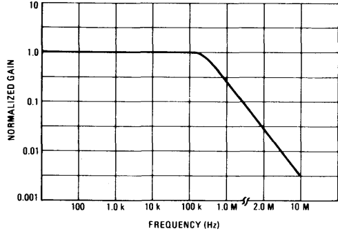
FIGURE 3 — NORMALIZED FREQUENCY RESPONSE
