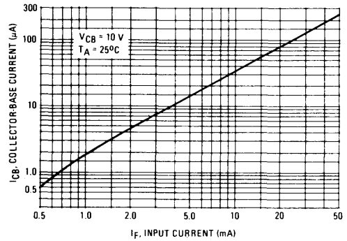
FIGURE 4 – COLLECTOR-BASE CURRENT versus INPUT CURRENT
