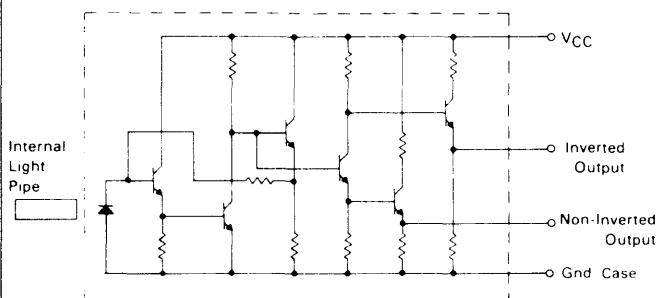
FIGURE 1 — EQUIVALENT SCHEMATIC
