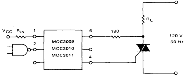
FIGURE 8 – RESISTIVE LOAD
