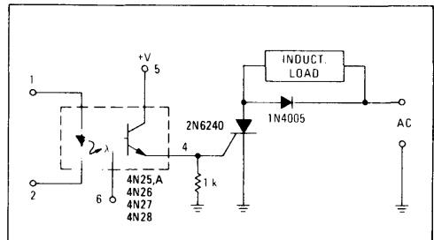
FIGURE 15 – INTERFACE BETWEEN LOGIC AND LOAD
