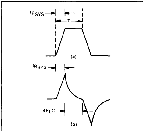
FIGURE 13 — Differentiator Waveforms
