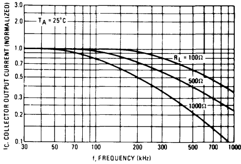
FIGURE 10 – FREQUENCY RESPONSE
