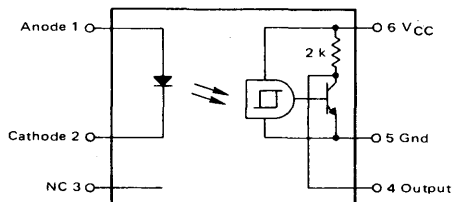
FIGURE 1 – COUPLER SCHEMATIC
