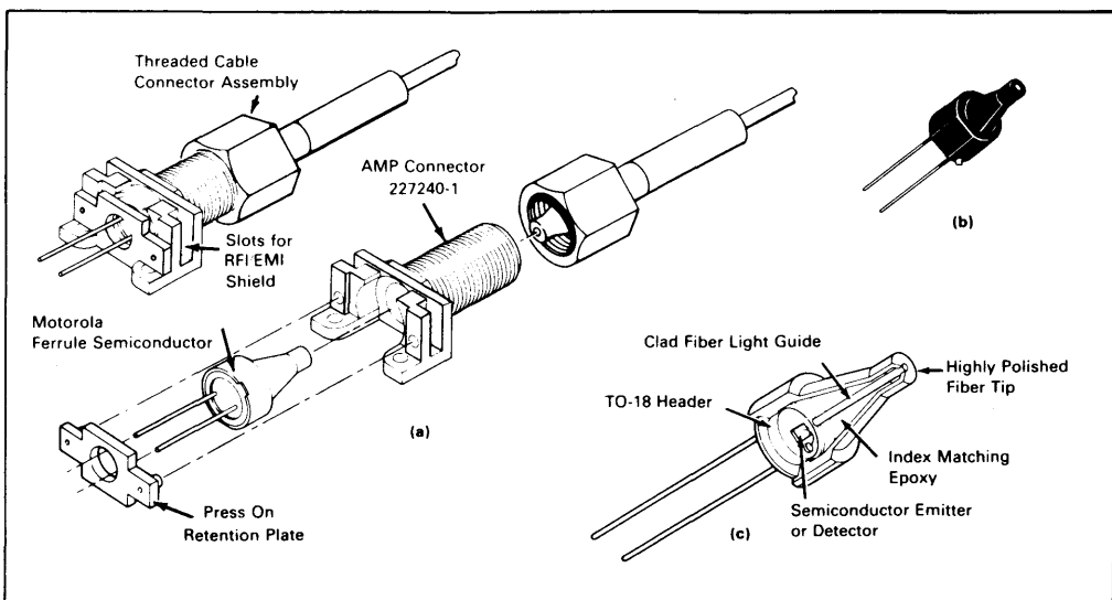
FIGURE 1 — Motorola Fiber Optic Active Component (FOAC)
