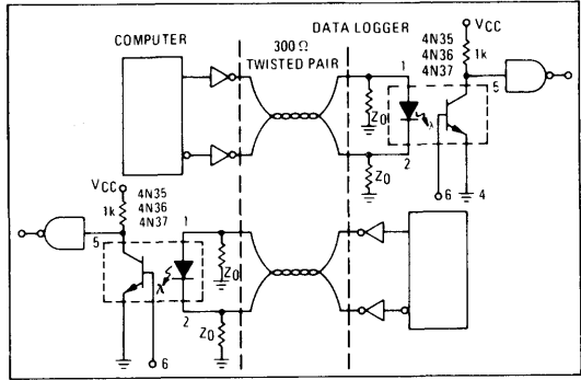
FIGURE 8 – COMPUTER/PERIPHERAL INTERCONNECT
