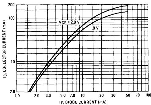
FIGURE 8 – MOC8050
