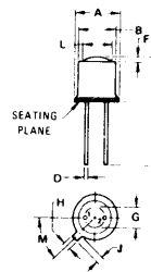
STYLE 1 PIN 1 ANODE PIN 2 CATHODE
