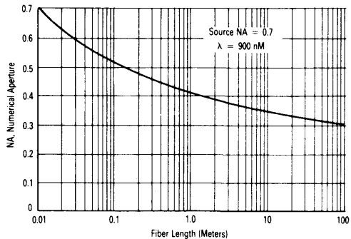
FIGURE 9 — NA versus Length for a Sample Fiber
