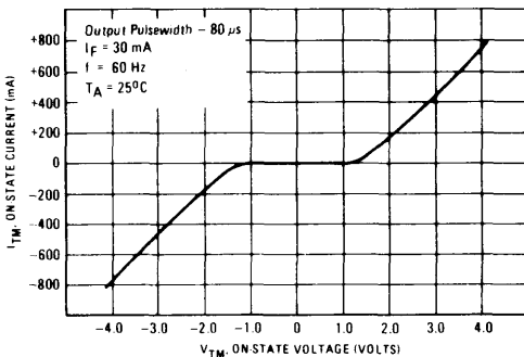
FIGURE 1 – ON-STATE CHARACTERISTICS
