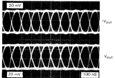
MFOD404F response to pseudo-random bit stream input with average optical input power of 1.0 microwatt. Note the good quality eye pattern at 10 Mbits per second. V_{CC} = 5.0\text{ V} .
