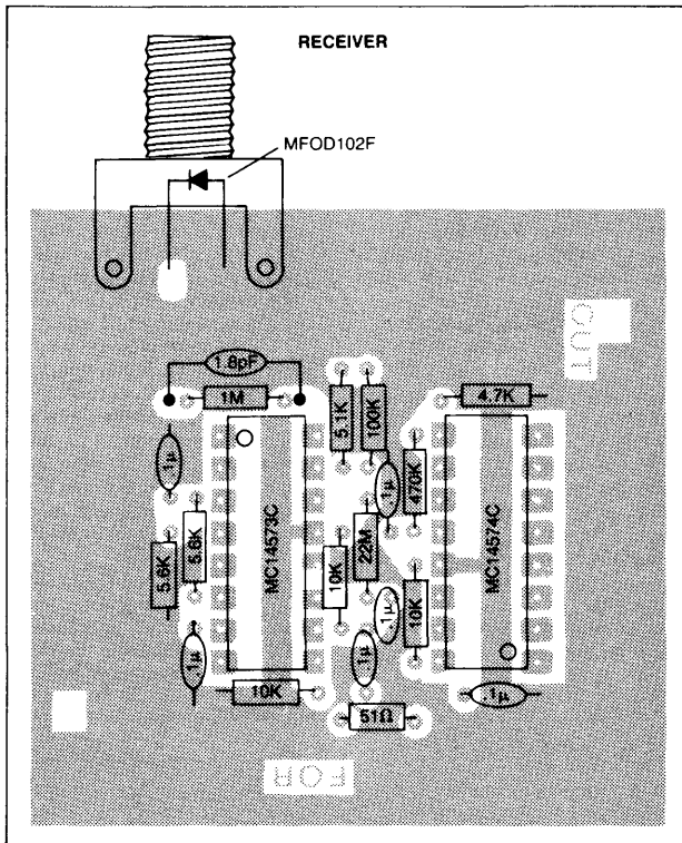
COMPONENT LAYOUT FIGURE 6.
