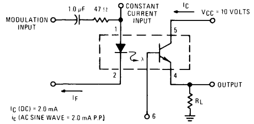
FIGURE 10 – FREQUENCY RESPONSE
