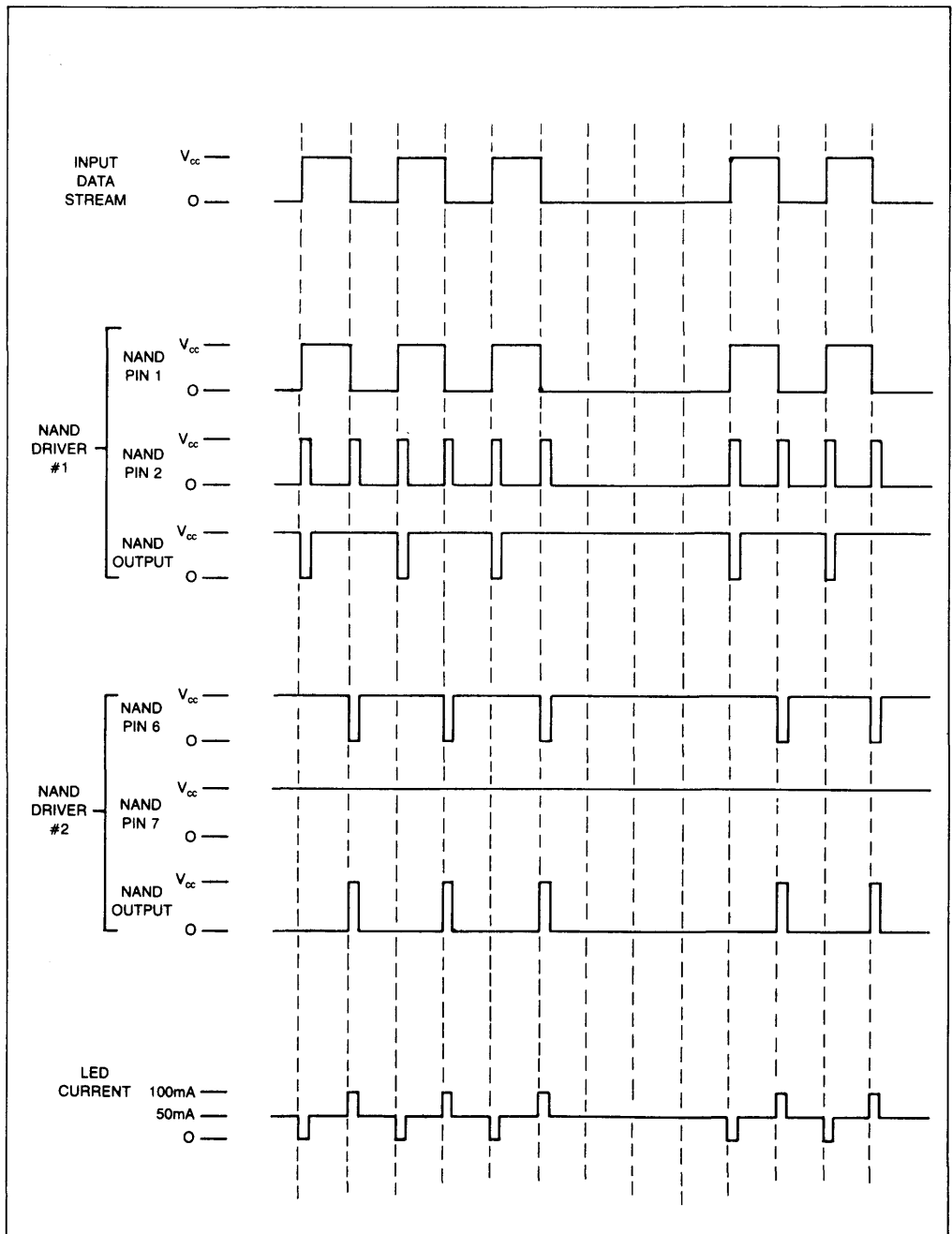
CIRCUIT WAVEFORMS FIGURE 4.
