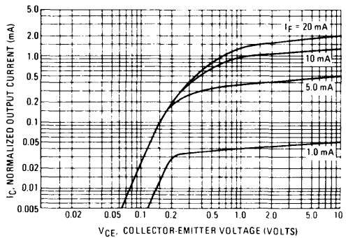
FIGURE 6 – COLLECTOR CHARACTERISTICS
