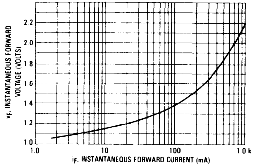
FIGURE 2 – FORWARD CHARACTERISTICS
