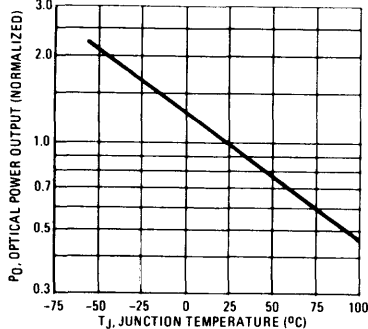
FIGURE 4 – OPTICAL POWER OUTPUT versus JUNCTION TEMPERATURE
