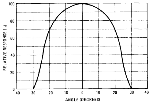
FIGURE 8 – ANGULAR RESPONSE
