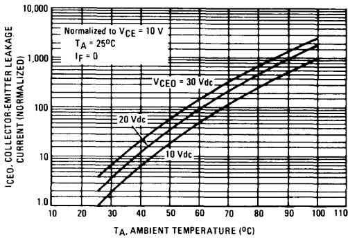
FIGURE 5 – COLLECTOR LEAKAGE CURRENT versus TEMPERATURE
