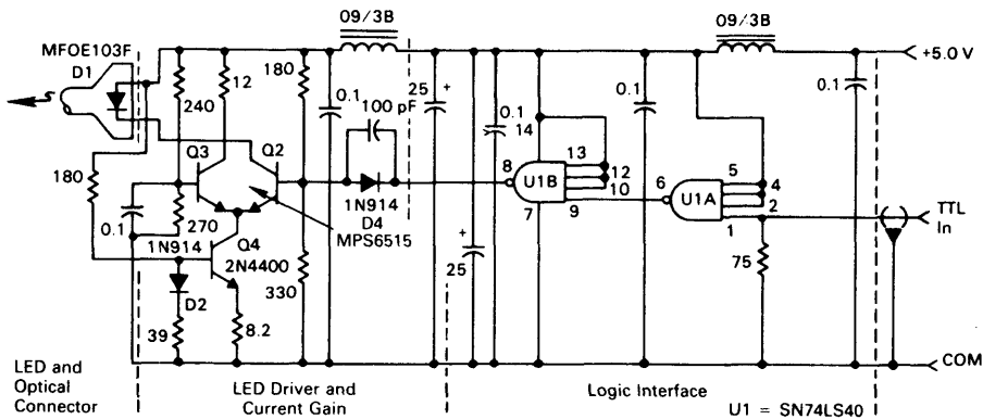
FIGURE 3 — Transmitter Schematic
