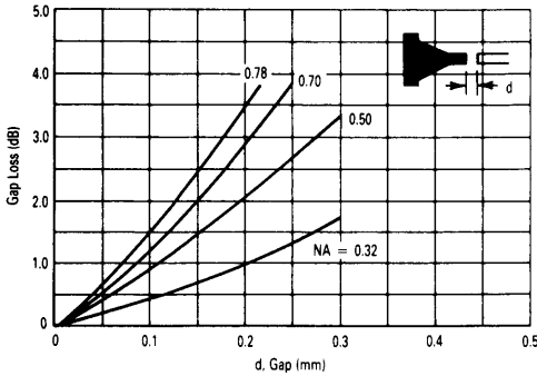
FIGURE 13 — Gap Loss
