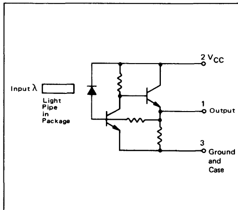
FIGURE 2 – EQUIVALENT SCHEMATIC
