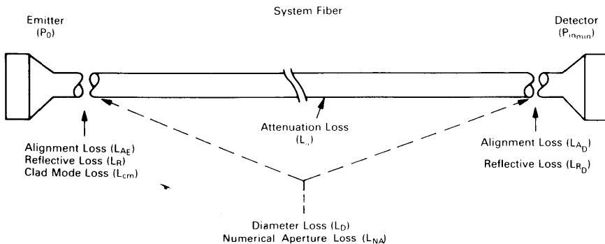
FIGURE 28 — Components of Loss Budget
