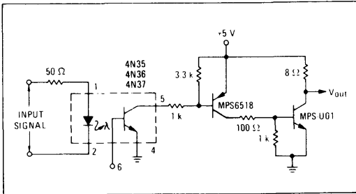
FIGURE 9 – POWER AMPLIFIER
