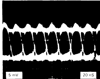
Eye-pattern generated by pseudo-random bit stream at 40 Mb/s
