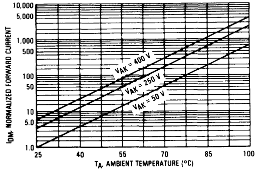
FIGURE 4 — FORWARD LEAKAGE CURRENT versus TEMPERATURE
