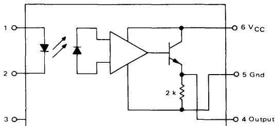
FIGURE 1 – COUPLER SCHEMATIC
