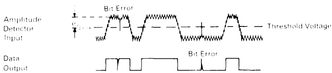
(a) Single-Ended ac-Coupled Data and Noise with Fixed Threshold at 50% Level
