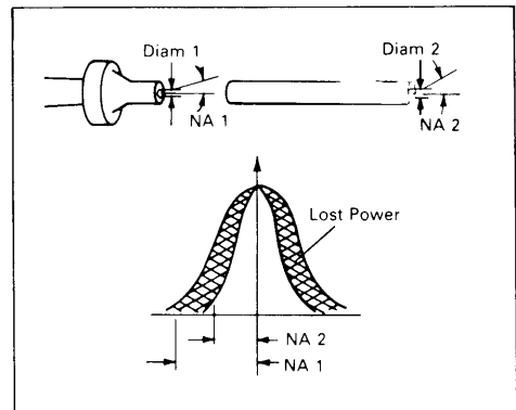
FIGURE 12 — NA Loss
