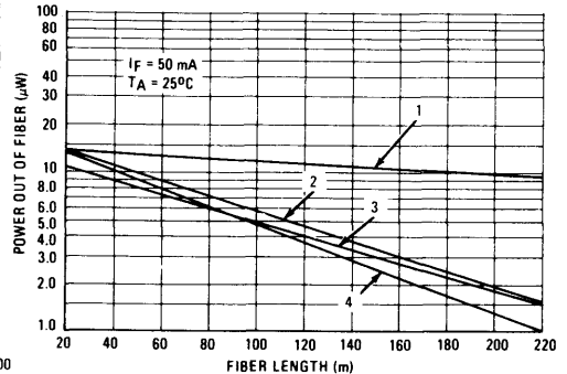
FIGURE 3 – POWER OUT OF FIBER* versus FIBER LENGTH
