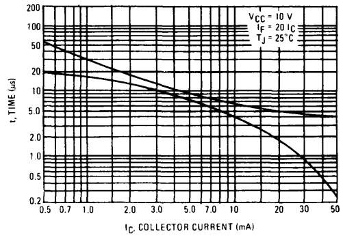
FIGURE 7 – TURN-OFF TIME
