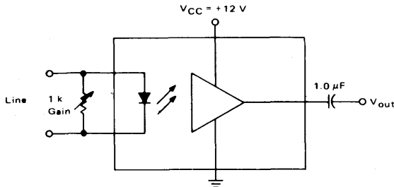
FIGURE 4 — TELEPHONE COUPLER APPLICATION
