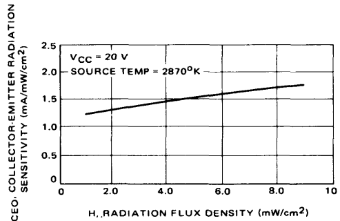
FIGURE 14 - Open Base Sensitivity versus Radiation for MRD300
