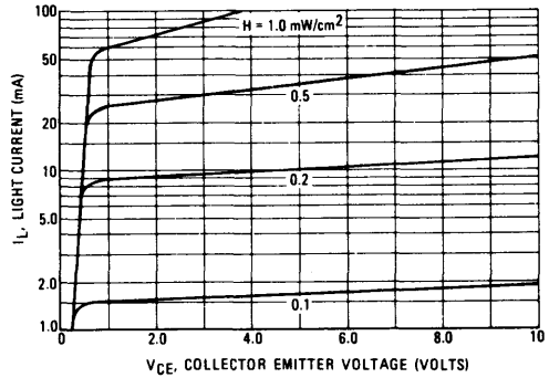
FIGURE 3 – COLLECTOR CHARACTERISTICS
