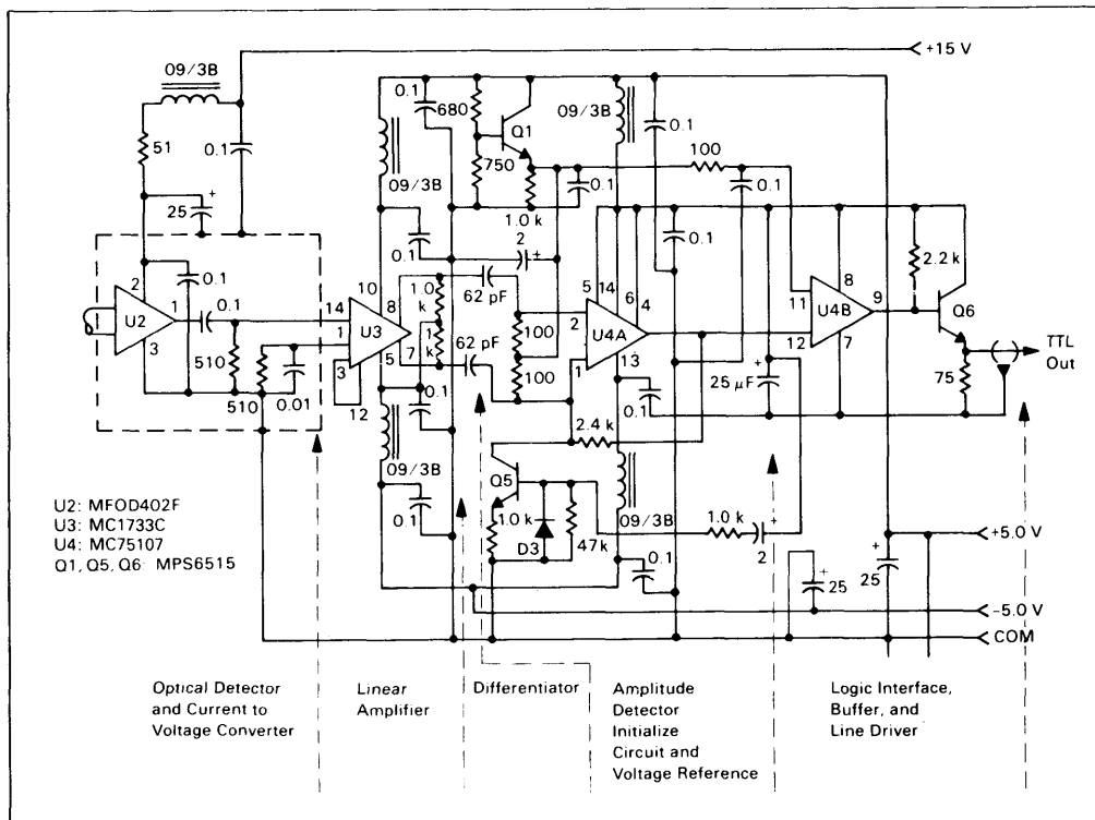
FIGURE 17 — Receiver Schematic
