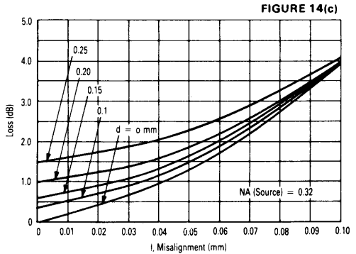
FIGURE 14 — Misalignment Loss
