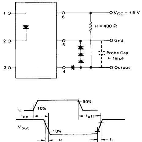
FIGURE 3 – TEST CIRCUIT
