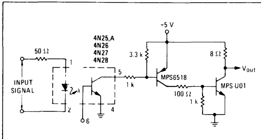
FIGURE 14 – POWER AMPLIFIER
