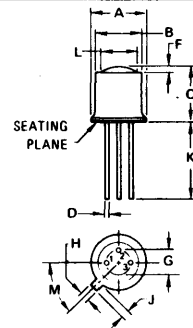
STYLE 3: PIN 1. MAIN TERMINAL PIN 2. MAIN TERMINAL PIN 3. SUBSTRATE (do not connect)
