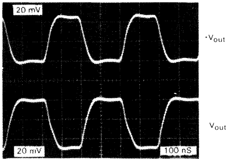
Pulse response of MFOD404F to square wave input with peak optical input power of 2.0 microwatts at V_{CC} = 5.0\text{ V}
