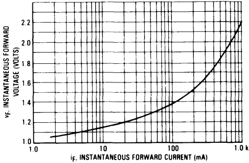
FIGURE 1 — FORWARD VOLTAGE versus FORWARD CURRENT
