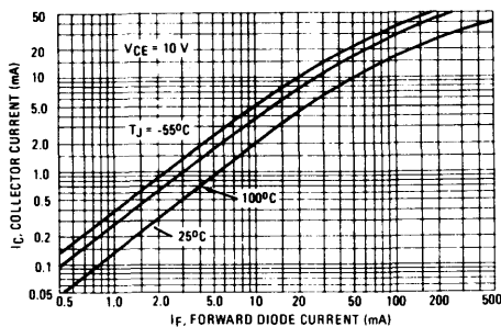
FIGURE 2 — 4N25, A, 4N26
