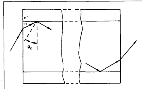
FIGURE 16 – Refraction in an Optical Fiber
