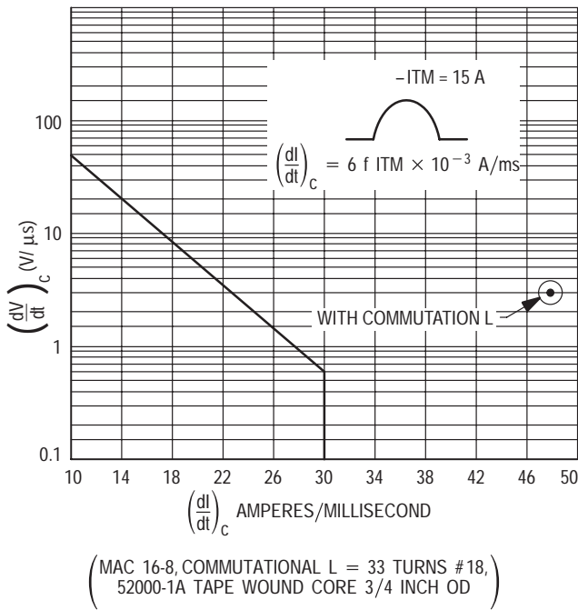
Figure 6.26. (\frac{dV}{dt})_c versus (\frac{dl}{dt})_c T_J = 125^\circ\text{C}
