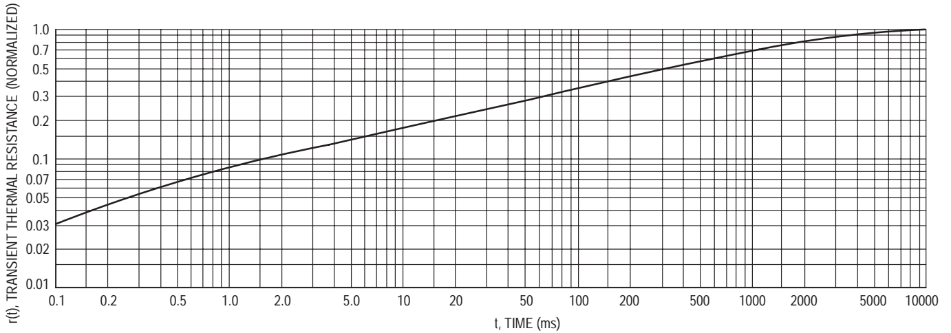
Figure 4. Thermal Response
