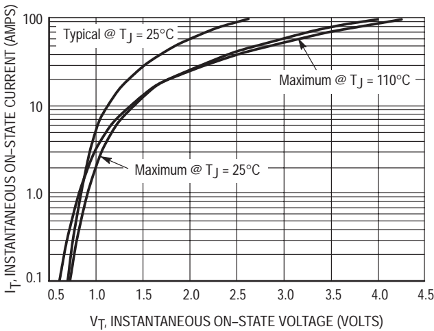
Figure 3. On-State Characteristics
