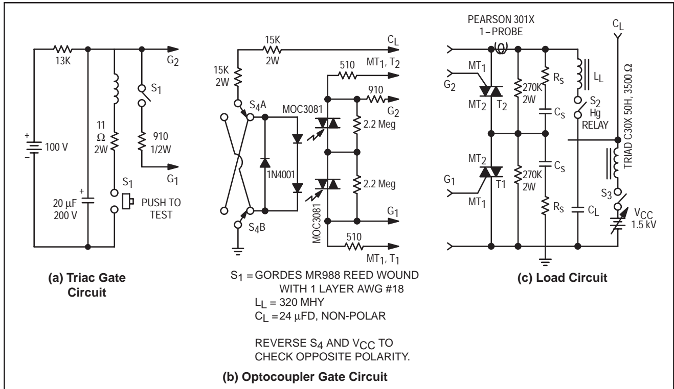
Figure 6.11. (\frac{dV}{dt})_c Test Circuit
