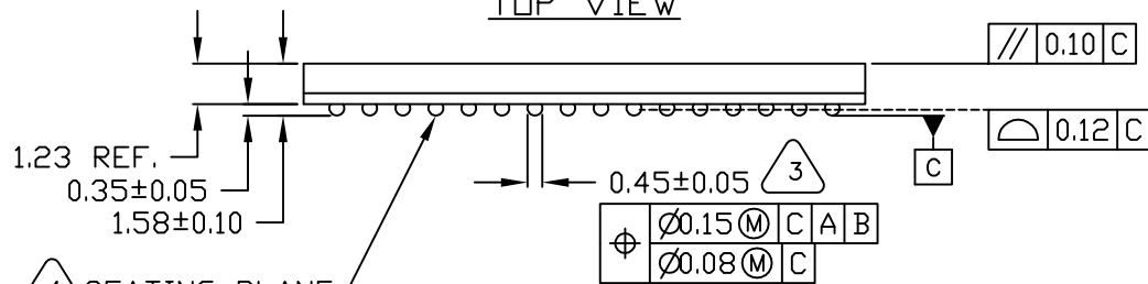
SIDE VIEW
