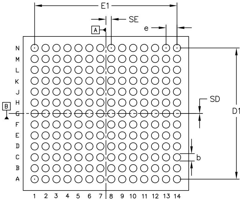
BOTTOM VIEW
