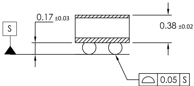
J-J' CROSS SECTION
