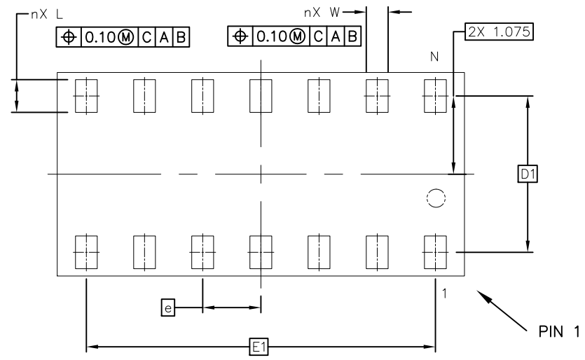
BOTTOM VIEW
