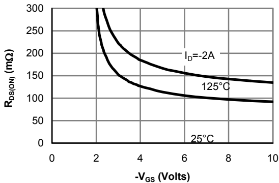
Figure 5: On-Resistance vs. Gate-Source Voltage
