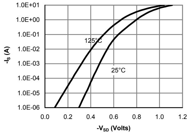
Figure 6: Body-Diode Characteristics
