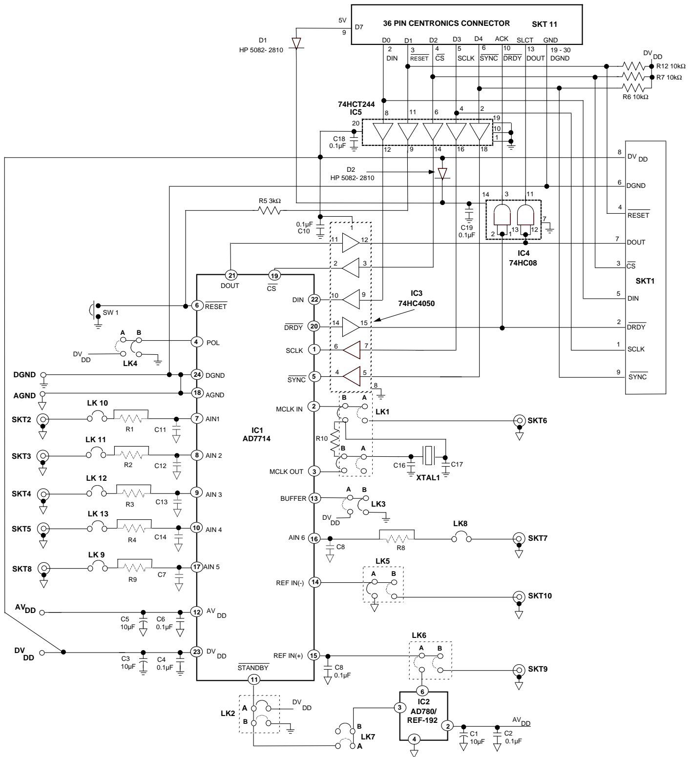
Figure 3. AD7714-5 Evaluation Board Circuit Diagram
