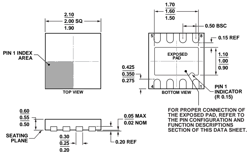
Figure 58. 8-Lead Lead Frame Chip Scale Package [LFCSP_UD] 2 mm x 2 mm Body, Ultra Thin, Dual Lead (CP-8-10)
