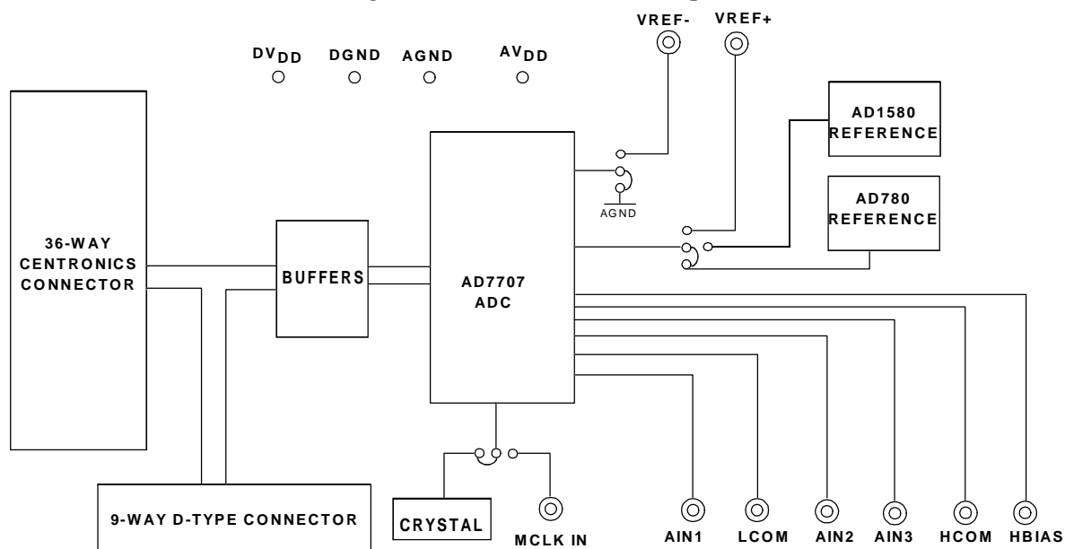
Figure 1: Evaluation Board Setup
