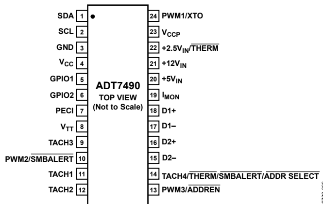
Figure 3. Pin Configuration
