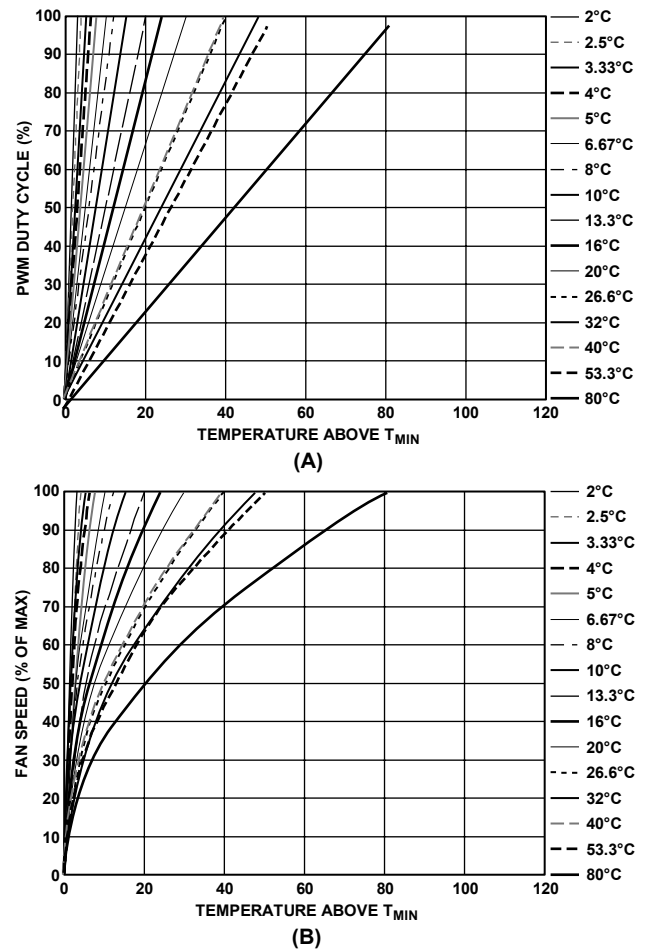
Figure 58. T_{RANGE} vs. Actual Fan Speed (Not PWM Drive) Profile
