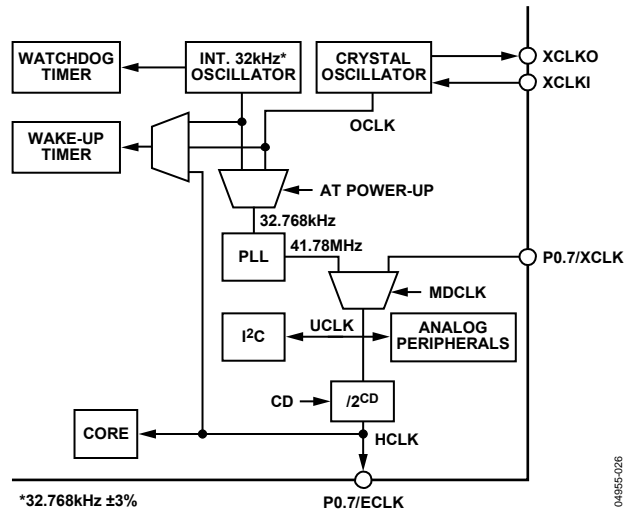
Figure 57. Clocking System
