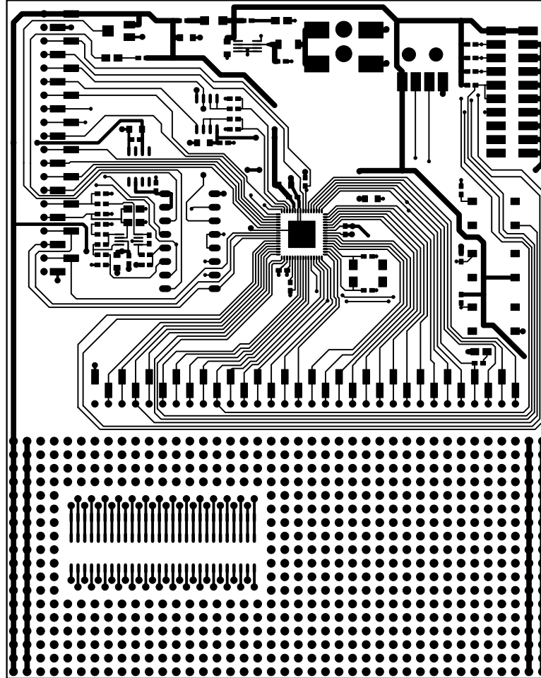
ADuC7024 EVALUATION BOARD Rev. B1 - Component Side View
