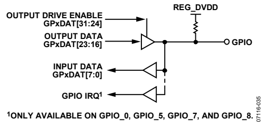
Figure 37. ADuC7034 GPIO
