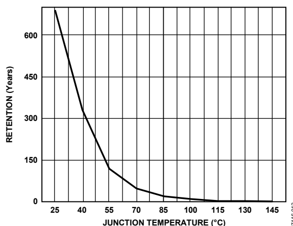
Figure 14. Flash/EE Memory Data Retention
