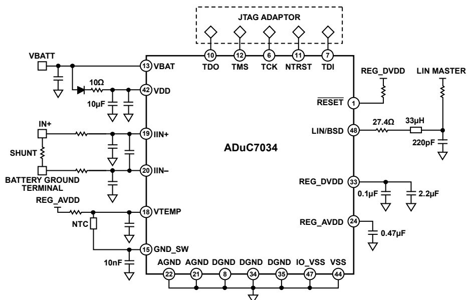
Figure 57. Schematic
