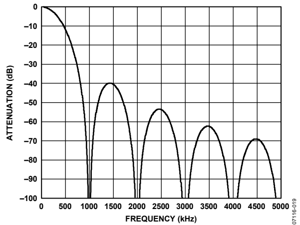
Figure 21. Typical Digital Filter Response at f_{ADC} = 1 \text{ kHz} (ADCFLT = 0x0007)
