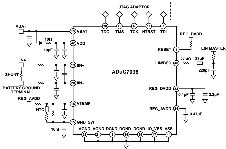
Figure 57. Simplified Schematic
