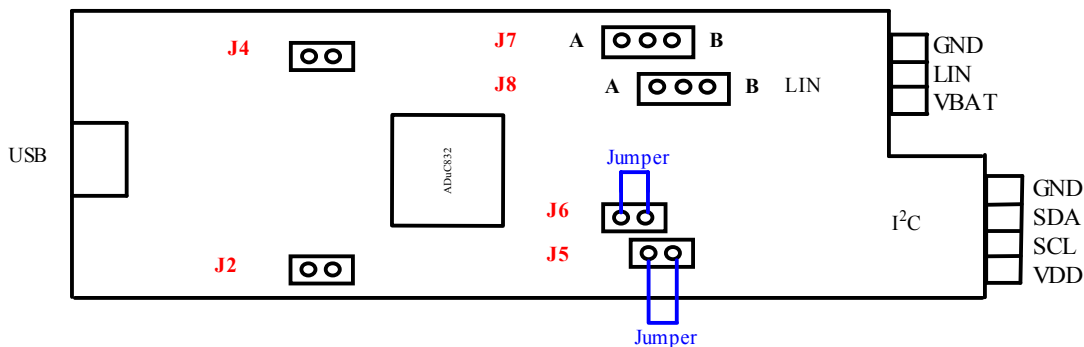
Figure 2 - LIN Jumper Settings
