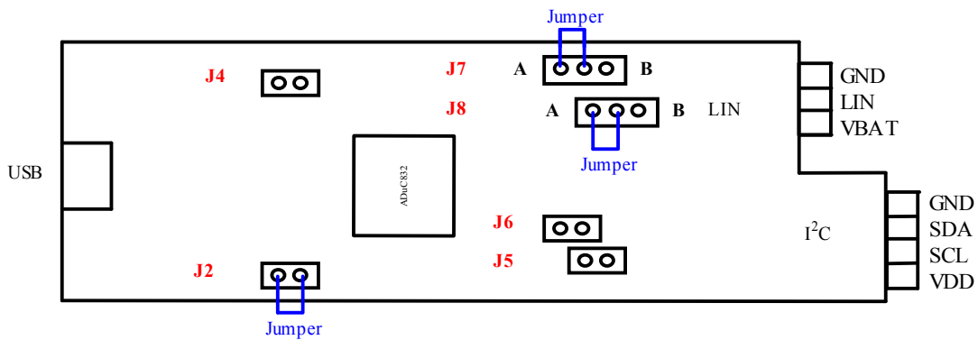
Figure 1 - I 2 C Jumper Settings (Default)
