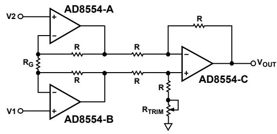
Figure 67. A Discrete Instrumentation Amplifier Configuration
