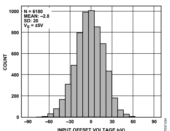
Figure 34. Input Offset Voltage Distribution, V_S = \pm 5V
