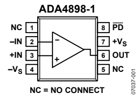
Figure 1. 8-Lead SOIC_N_EP (RD-8-1)
