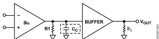
Figure 40. Topology
