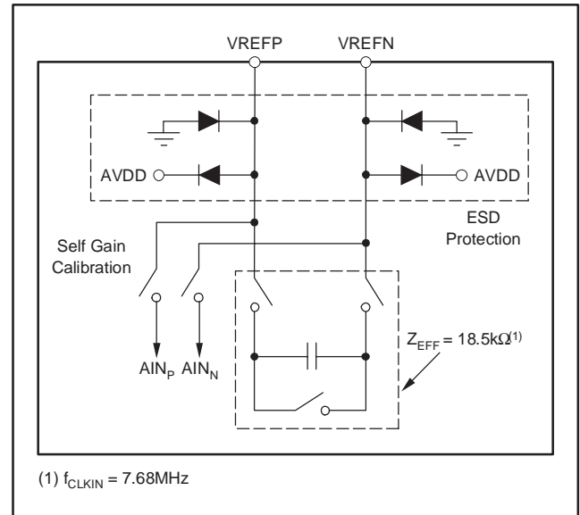
Figure 12. Simplified Reference Input Circuitry
