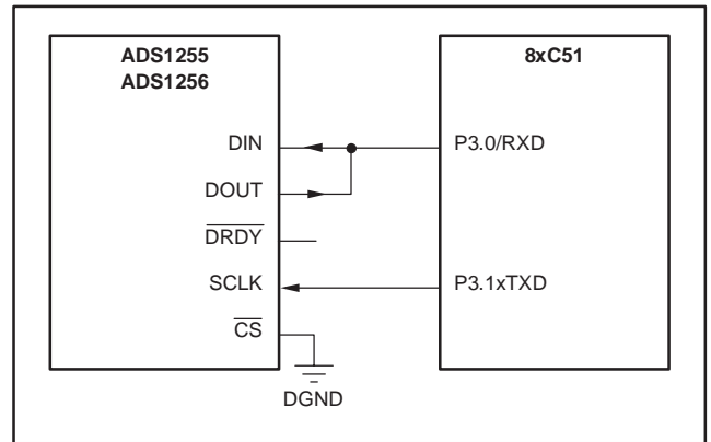
Figure 28. Connection to 8xC51 Microcontroller UART with a 2-Wire Interface
