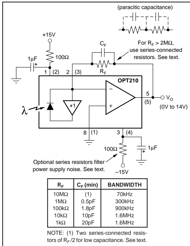
FIGURE 1. Basic Operation.
