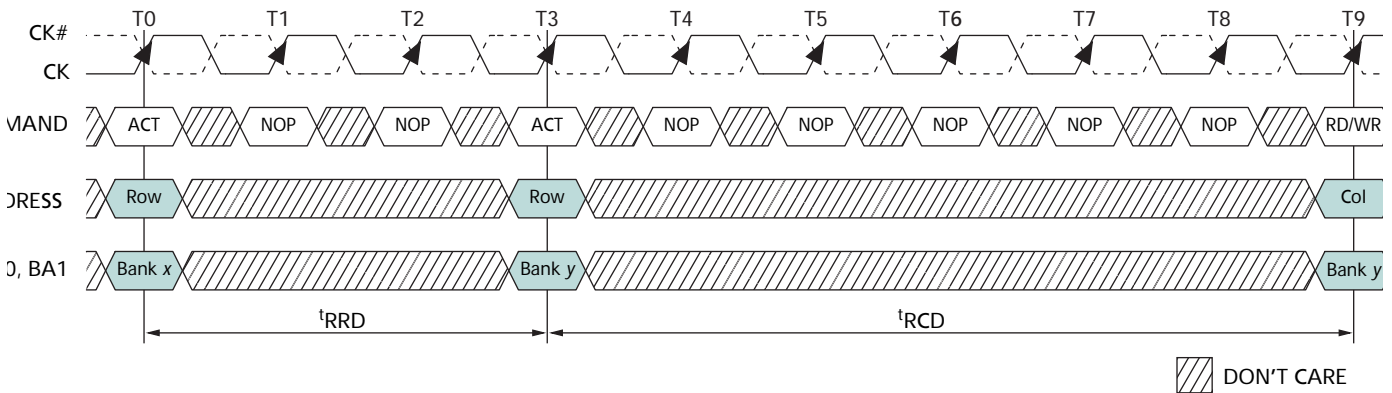
Figure 17: Example: Meeting t_{RRD} (MIN) and t_{RCD} (MIN)
