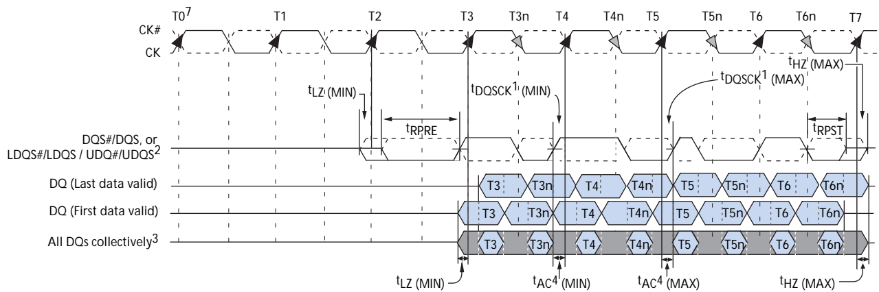
Figure 29: Data Output Timing – t_{AC} and t_{DQSCK}
