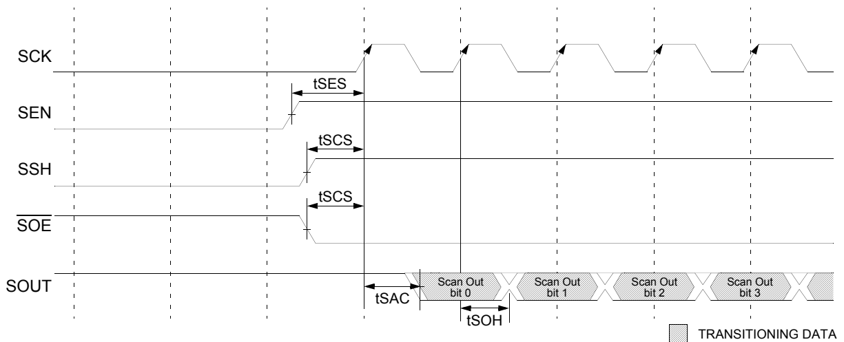
Figure 3. Scan Shift Timing
