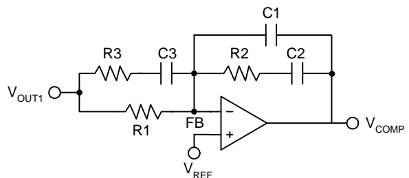
Figure 6. Compensation Network
