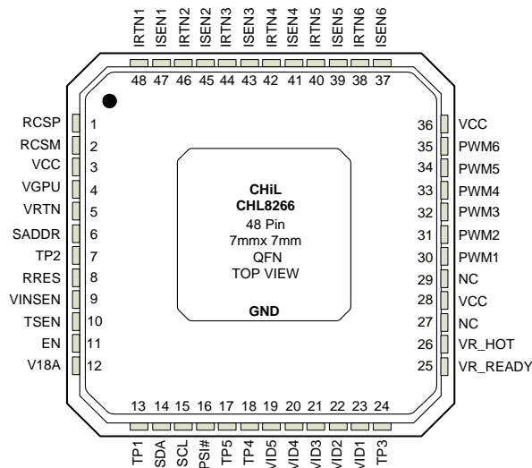
Figure 1. CHL8266 48 Pin QFN Package
