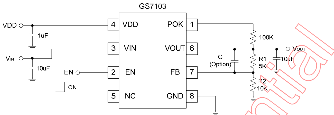
Figure 1 Typical Application of GS7103
