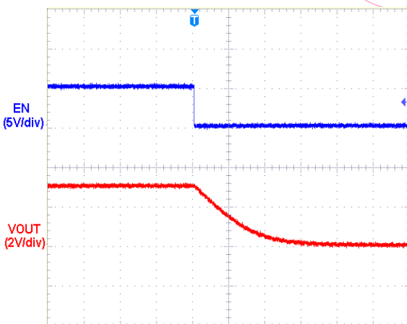
V OUT =3.0V, I OUT =0mA, V DD =4.0V
