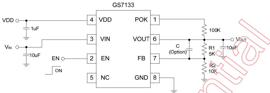
Figure1 Typical Application of GS7133
