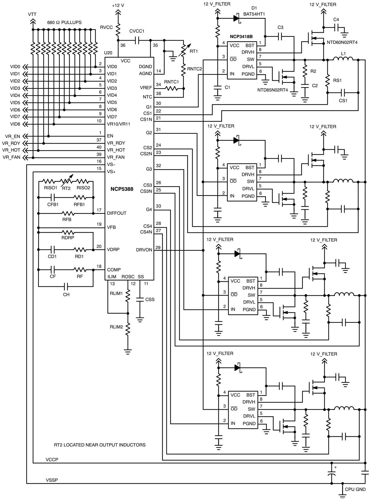
Figure 2. Application Schematic for Four Phases
