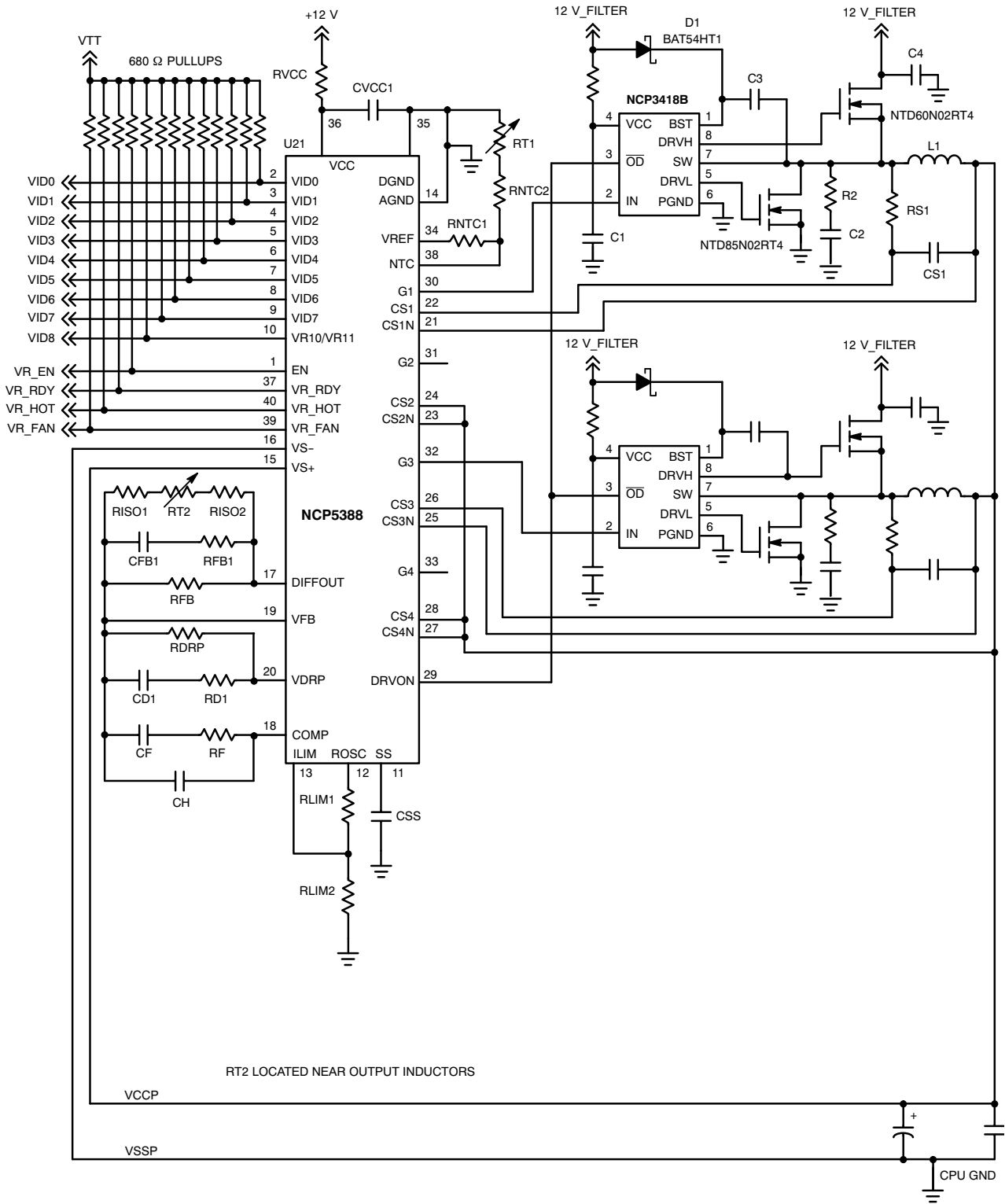
Figure 4. Application Schematic for Two Phases
