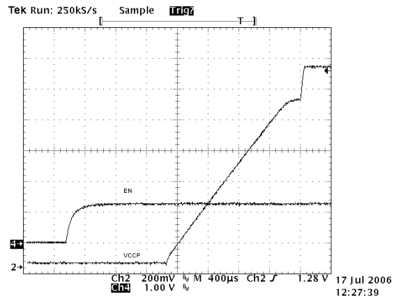
Figure 15. VR11 Startup
