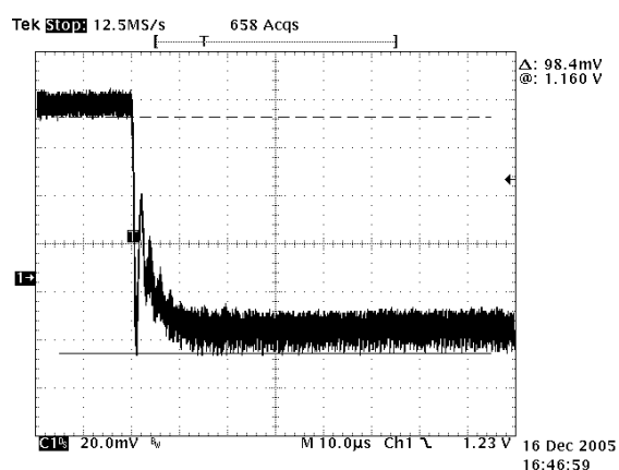
Figure 10. Typical Step Load Response
