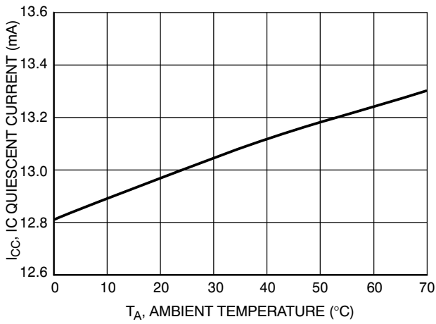
Figure 5. IC Quiescent Current vs. Ambient Temperature
