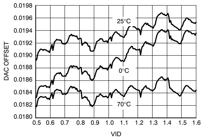
Figure 7. Typical DAC Voltage Offset vs. Temperature
