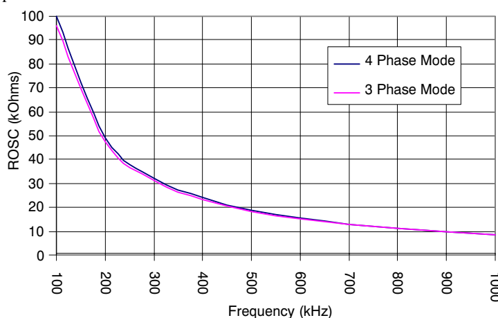
Figure 17. ROSC vs. Phase Frequency
