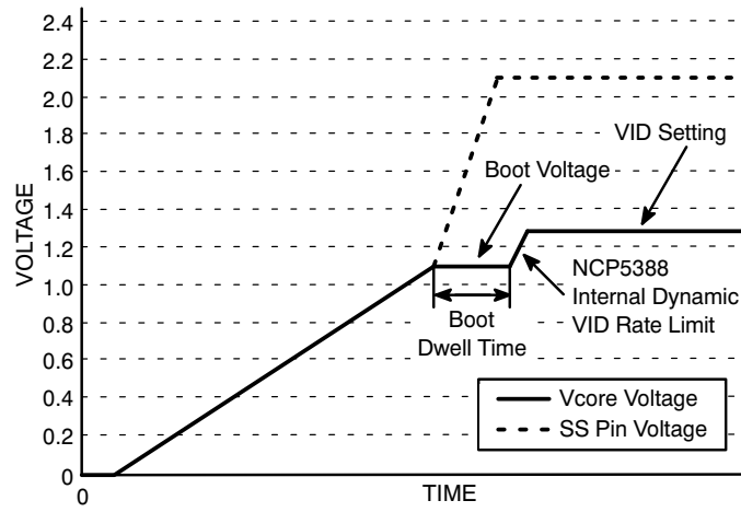
Figure 9. Typical VR11 Soft-Start Sequence to Vcore = 1.3 V
