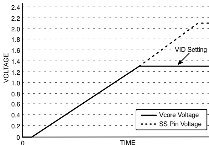
Figure 8. Typical VR10 Soft-Start Sequence to Vcore = 1.3 V
