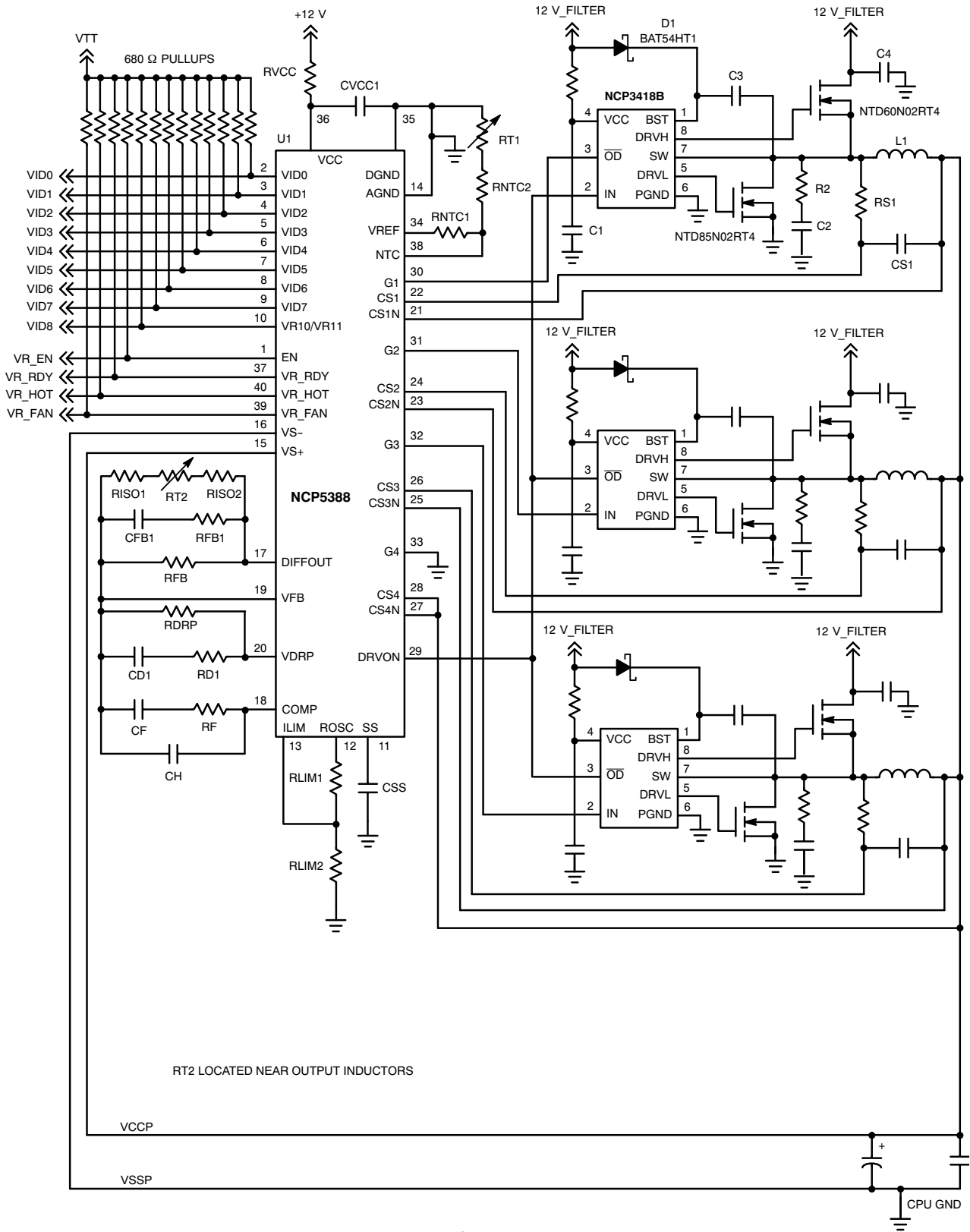
Figure 3. Application Schematic for Three Phases
