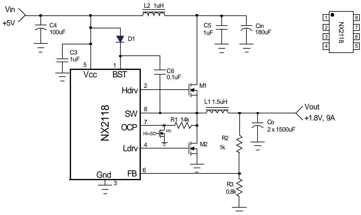
Figure1 - Typical application of 2118
