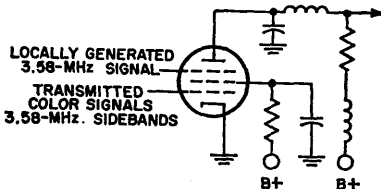
Fig. 97—Low-level color demodulator.
