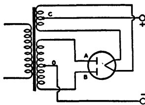
Fig. 126—Schematic diagram of full-wave rectifier tube and circuit connections.
