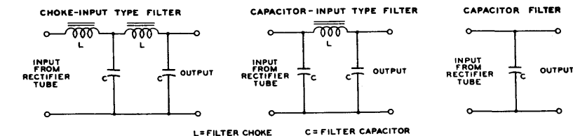
Fig. 121—Typical smoothing filters for rectifier tubes.
