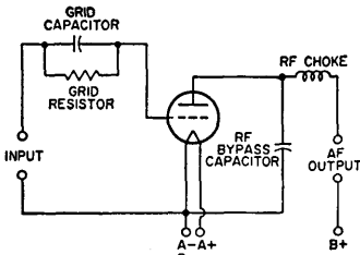
Fig. 27—Detector circuit using grid-resistor-and-capacitor bias.
