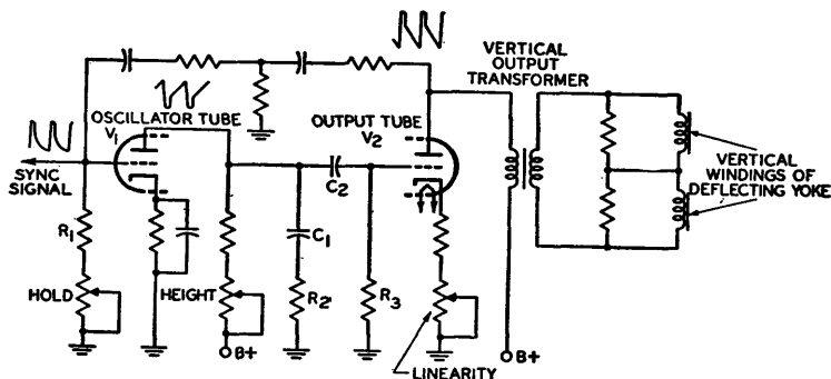
Fig. 90—Simplified combined vertical-oscillator-and-output stage.
