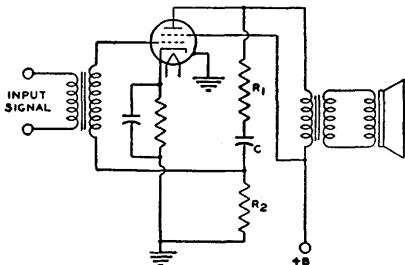
Fig. 48—Power-output stage using constant-voltage inverse feedback.
