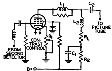
Fig. 76—Typical video amplifier stage.
