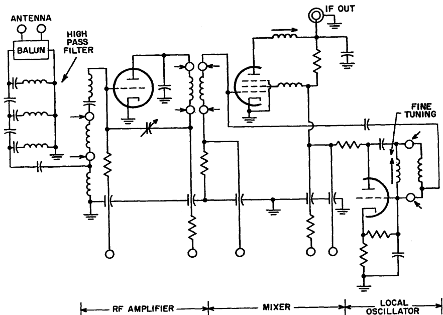
Fig. 72—Simplified schematic of typical vhf television tuner.
