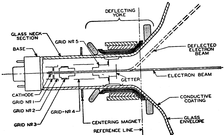
Fig. 10—Structure of television-picture-tube electron gun.
