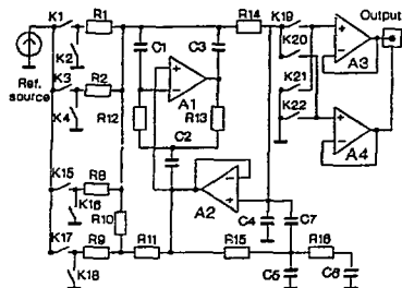
Fig.2. The analog section of multiphase PWM-DAC.
