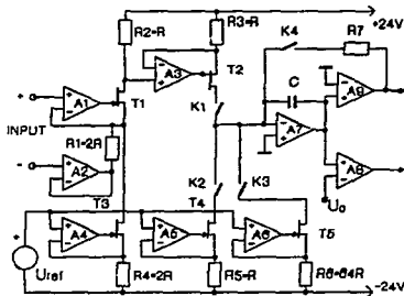
Fig. 3. Three-step integrating ADC.
