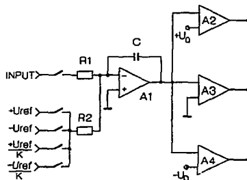
Fig. 4. ADC with multicycle integration.
