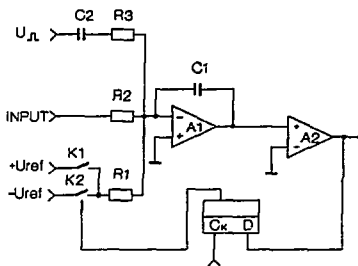
Fig.5. ADC with dynamic-integrator.
