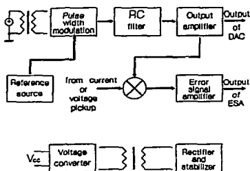
Fig.1. The analog section of PWM-DAC.
