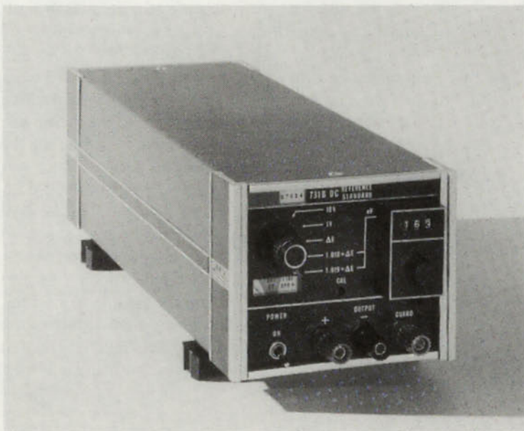
Figure 89. Fluke Model 731B D.C. Reference Standard.
