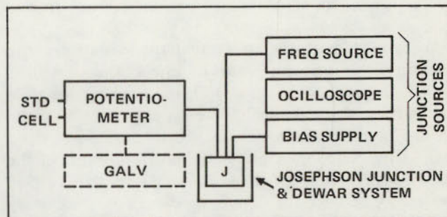
Figure 38. Block diagram of the overall voltage standard system, with a Josephson junction voltage reference for the potentiometer, which is used to calibrate standard cells.
