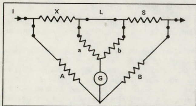
Figure 17. Kelvin double-bridge.
