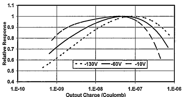
Figure 2. UV photodiode response at three different bias voltages. at 193 nm.
