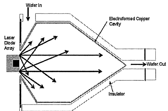
Figure 1. The figure shows a cutaway diagram of the FWOPM, illustrating the absorbing cavity and the water-flow channel on the outer surface of the cavity. The laser diode array is placed in the entrance aperture, and the cavity absorbs nearly 2π steradians of its optical output.
