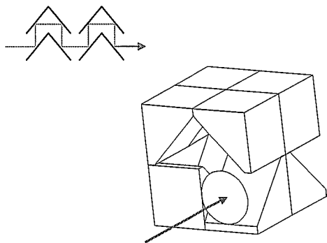
Figure 3. Representation of a reflective attenuator with 8 mirror surfaces. Inset shows schematically the light (indicated by arrow) is reflected at 45° angle of incidence. The input beam is coaxial with the output.
