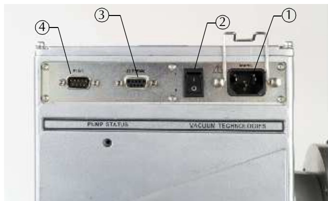
Figure 4 Inverter Interface
