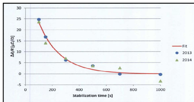
Fig. 1. Example of stabilization time with 1000 V test voltage for the 100 G \Omega primary standard resistor used at ICE.
